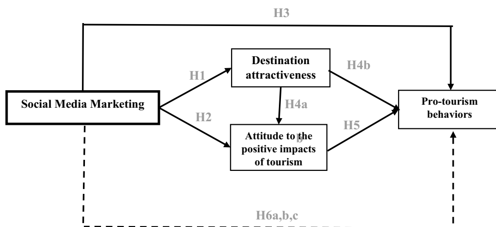
Fig. 1 Research framework
